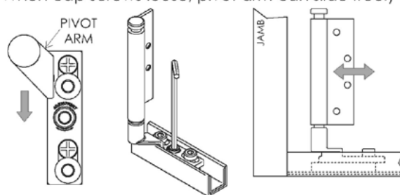
When cap screws loose, pivot arm can slide freely
