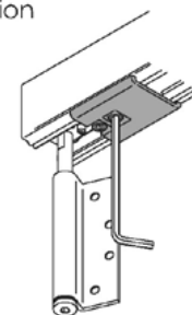
When cap screws loose, pivot arm can slide freely
