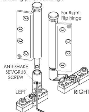
Handling pivot set hinge
