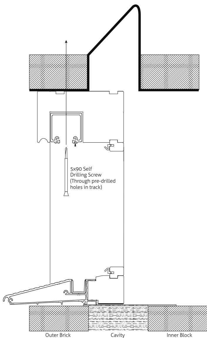
PRESSED STEEL LINTEL
